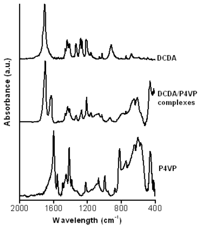
Figure S1. Infrared spectra of P4VP, DCDA, and DCDA/P4VP complexes at MR=1/1.
