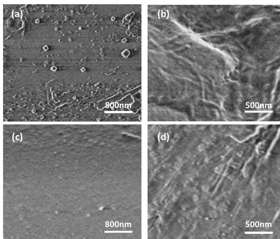
Figure S2. Comparison of the PPTA material colored by carbon black and MWCNT after treated in a NaOH aqueous solution (concentration of 1 mol/L) for two weeks under SEM. (a) and (b) The PPTA material colored by carbon black and MWCNTs, respectively. (c) and (d) Alkaline treatments of (a) and (b) for 2 weeks, respectively.
