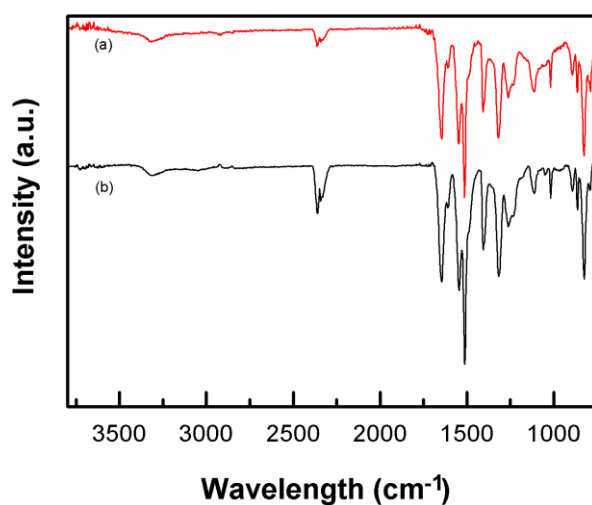
Figure S1. Fourier transform infrared spectra of (a) pristine PPTA and (b) colored PPTA stripes by MWCNTs with weight concentration of 5%.
